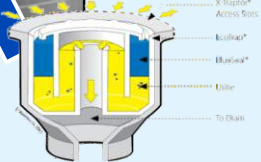
Cross-Section of EcoTrap®
